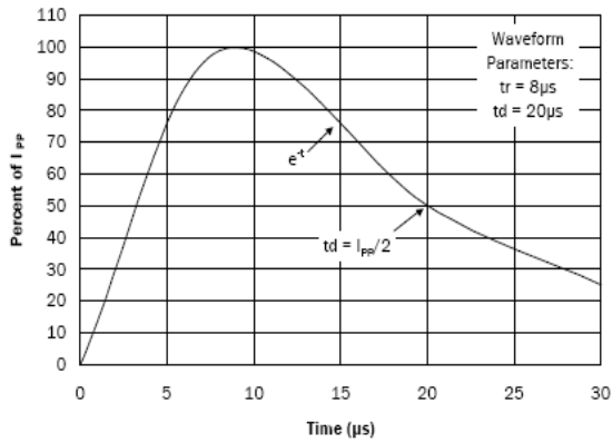
Pulse Waveform
