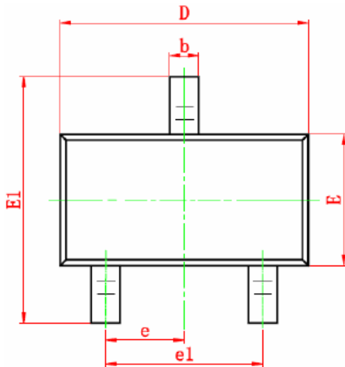
SOT23-3L PACKAGE DIAGRAMS TOP VIEW
